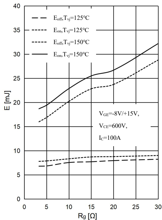
图 5 . IGBT 开关损耗-栅极电阻 Fig 5. IGBT Switching Loss E_{on} & E_{off} vs. R_g
