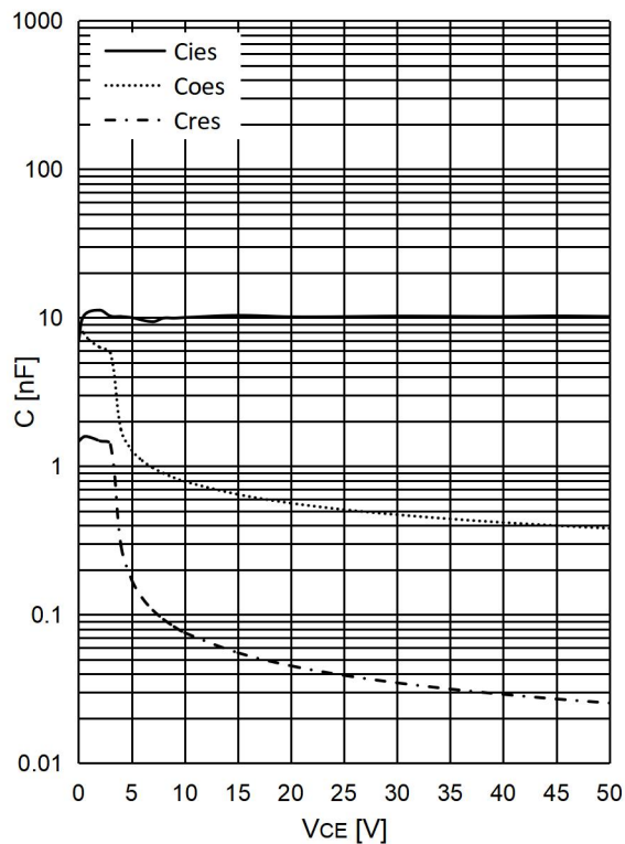
图 12.IGBT 电容特性 Fig 12.IGBT Capacity Characteristic
